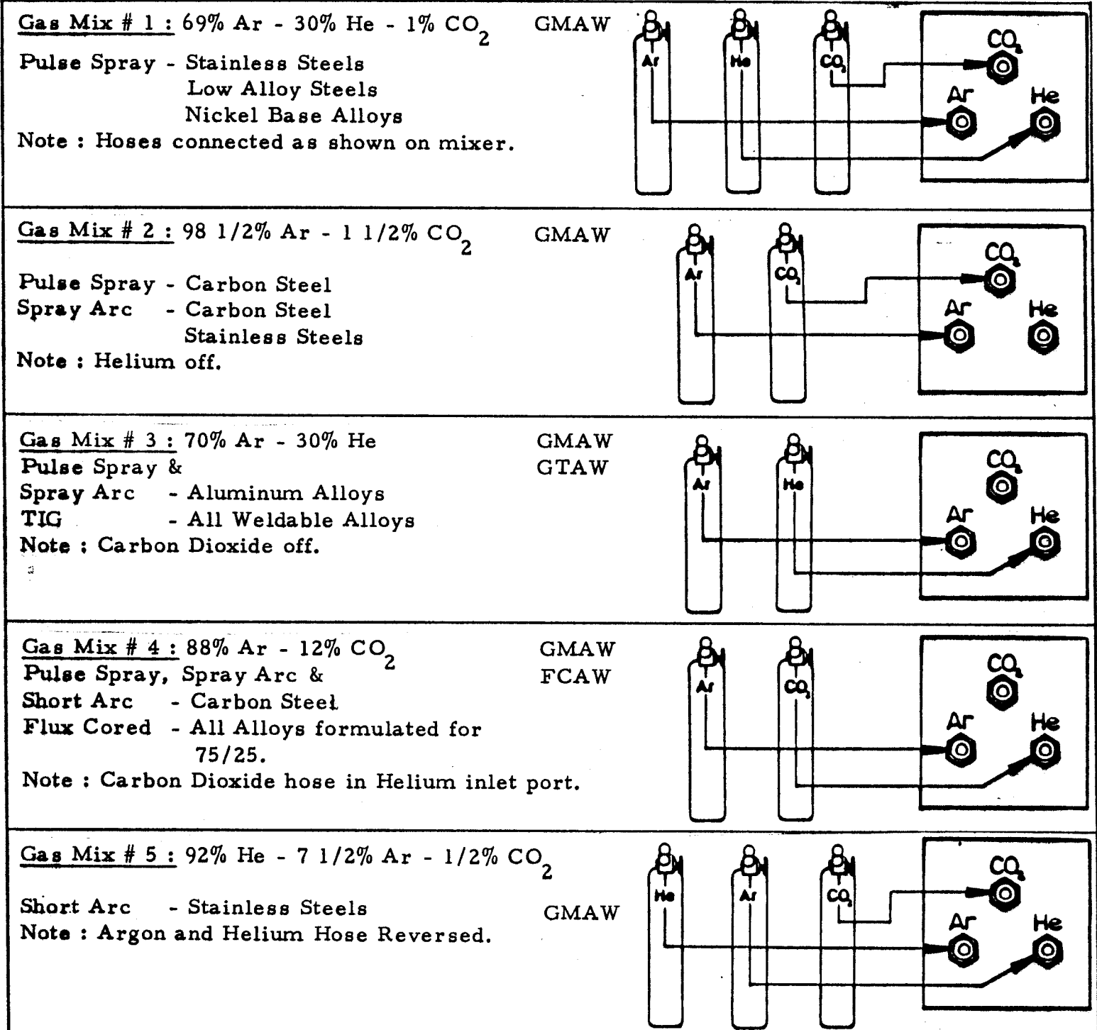
FIG-2 Hose Interchange Diagram
